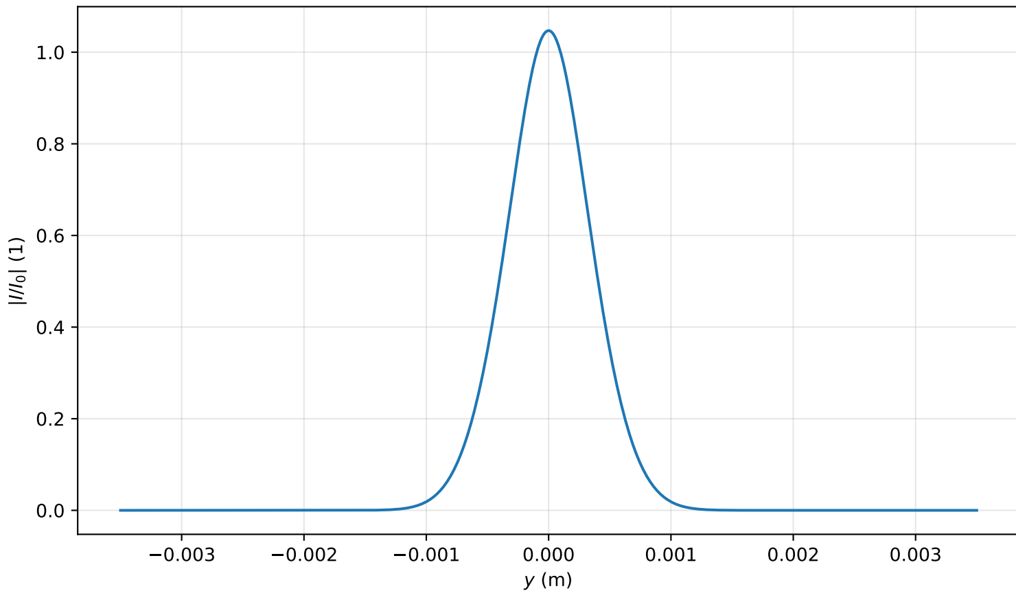
Intensity profile I(x = 0, y, z = 0.398)/I_0 , P_{in}=0.6P_{cr} , artificial time
